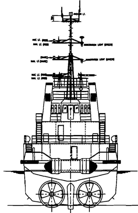
STERN VIEW
