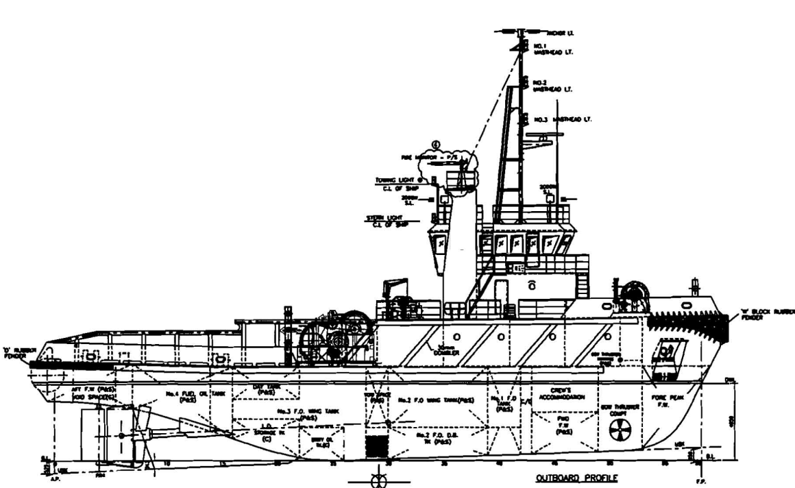
OUTBOARD PROFILE
