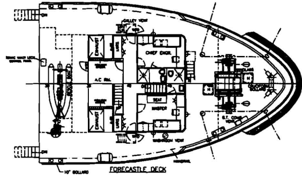
FORECASTLE DECK
