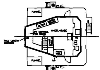
WHEELHOUSE DECK
