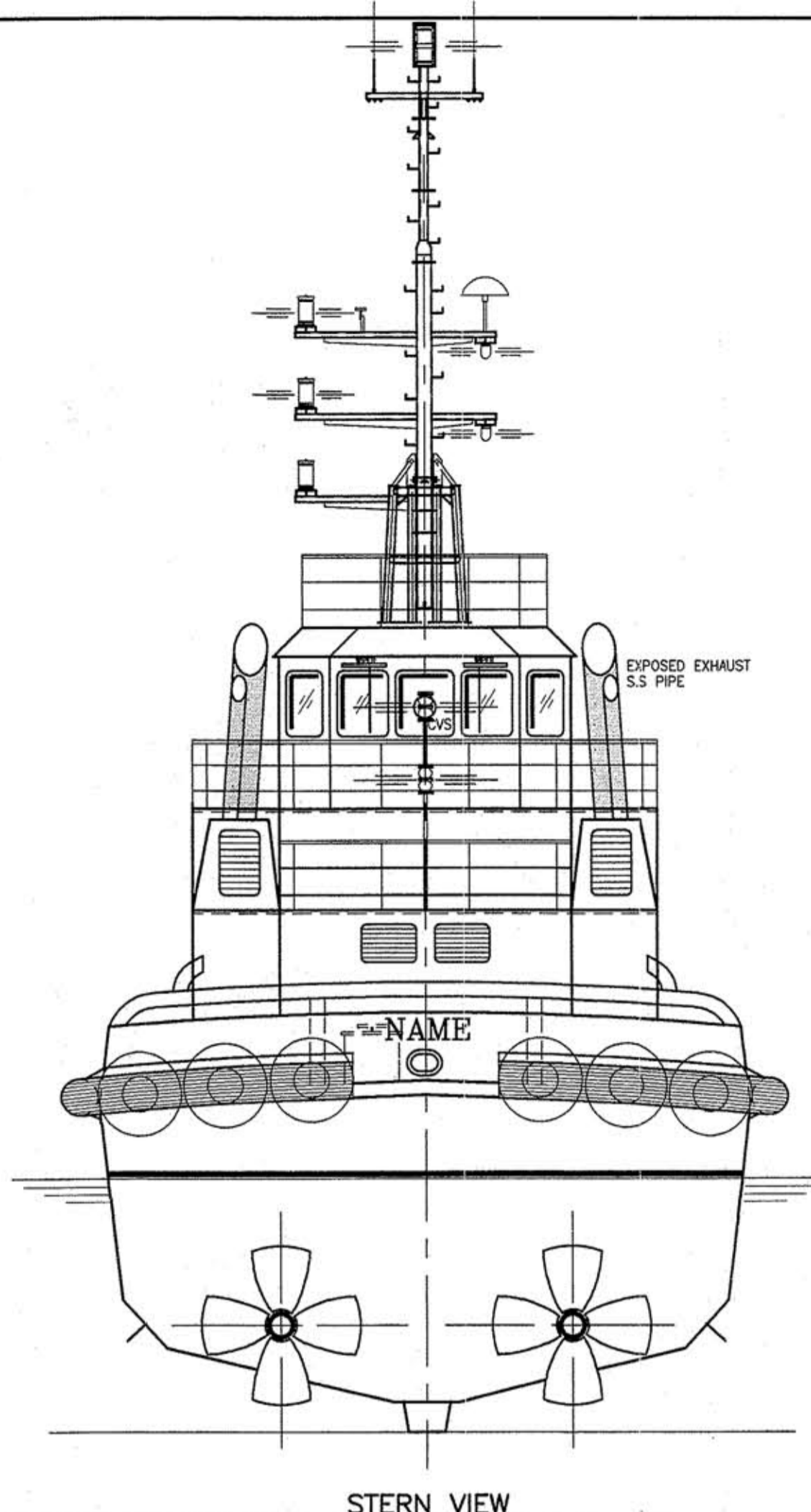
STERN VIEW
