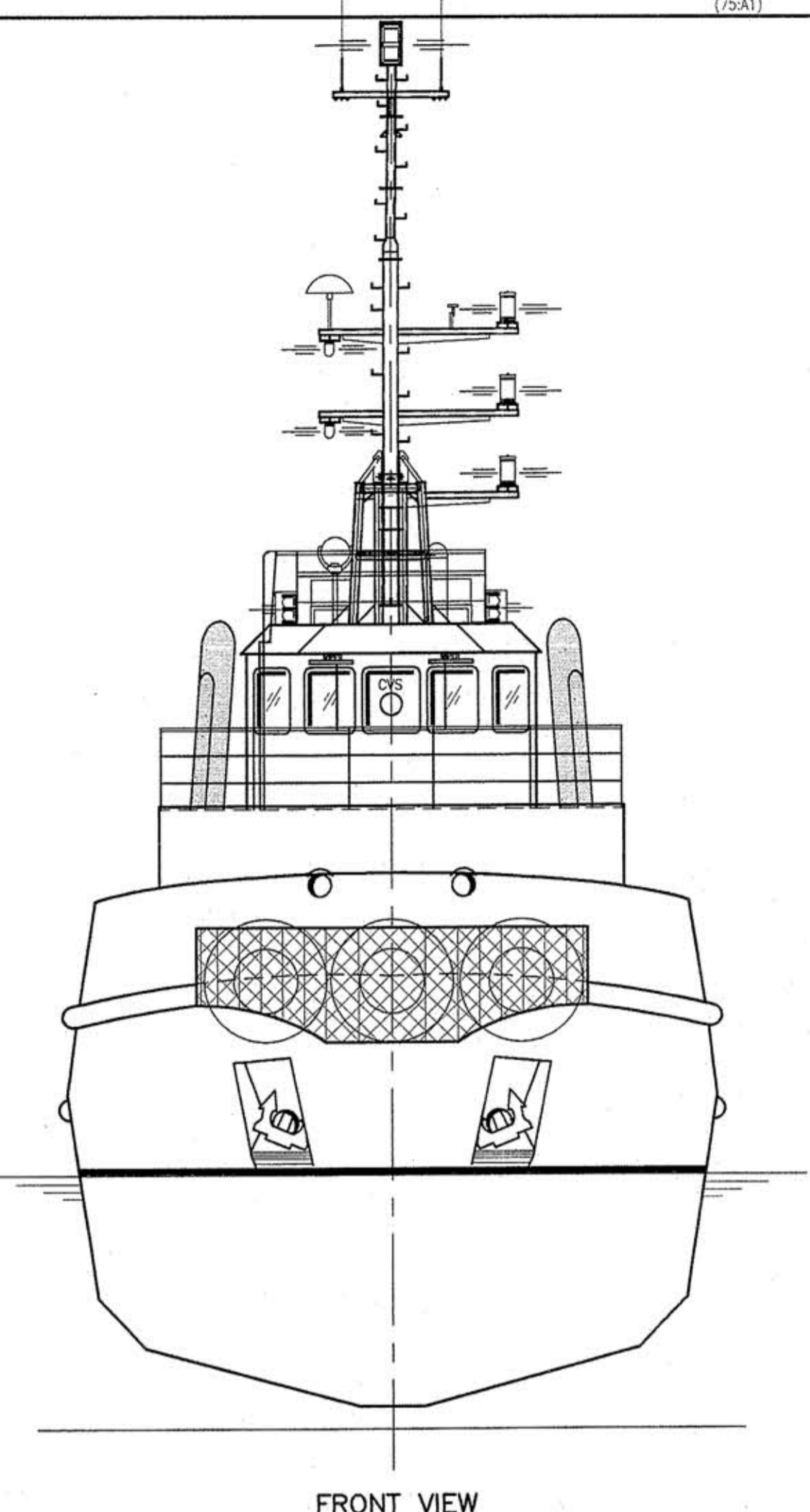
FRONT VIEW
