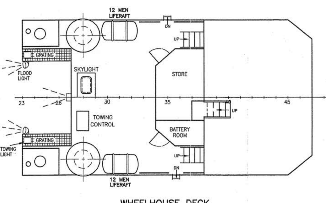
WHEELHOUSE DECK
